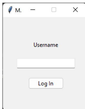
Figure 3: User’s Interface
